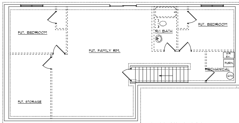
FOUNDATION PLAN
