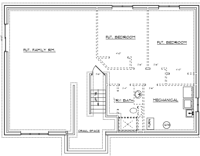
FOUNDATION PLAN
