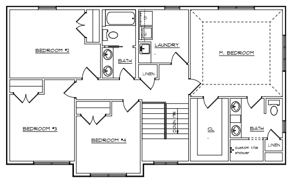
UPPER FLOOR PLAN 1018 sq.ft.
