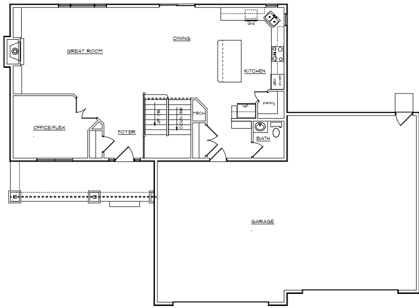
MAIN FLOOR PLAN 1001 sq.ft.
