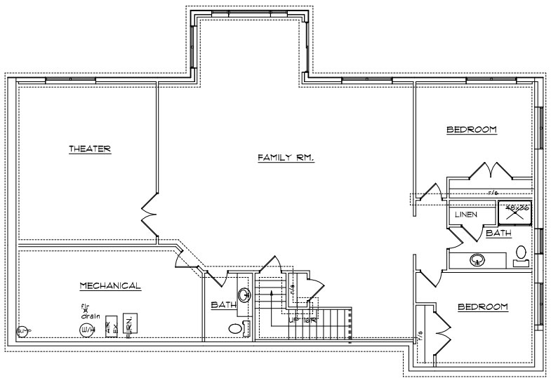
FOUNDATION PLAN 1800 sq.ft. finished
